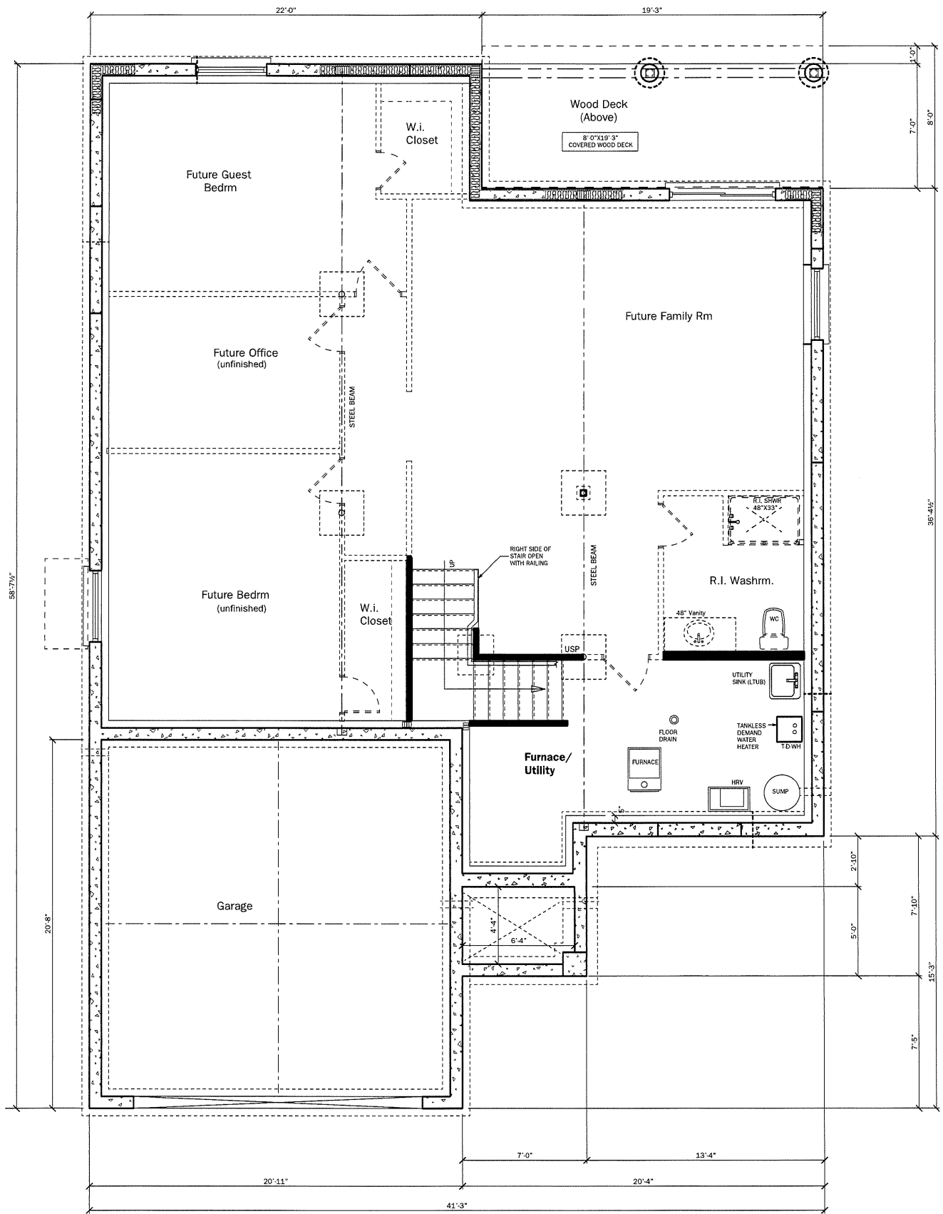
FOUNDATION / BASEMENT PLAN GLENWOOD #2 MODEL Rosewood Acres Phase 4
